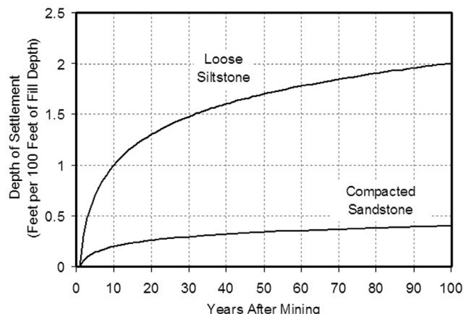
Figure 4. Estimated settlement of unsaturated mine fill with time, beginning one year after mining.
