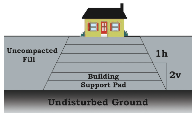
Figure 2. A representation of a mine-spoil pad constructed to support an intended building site during reclamation. The spoil pad should extend beyond the minimum area required to support the building. In most cases, the zone where the surface is compacted should extend at least 10 feet beyond the intended footing area. The compacted spoil pad should extend downward at a minimum angle of about 30 degrees from the vertical (a 2v:1h slope).
